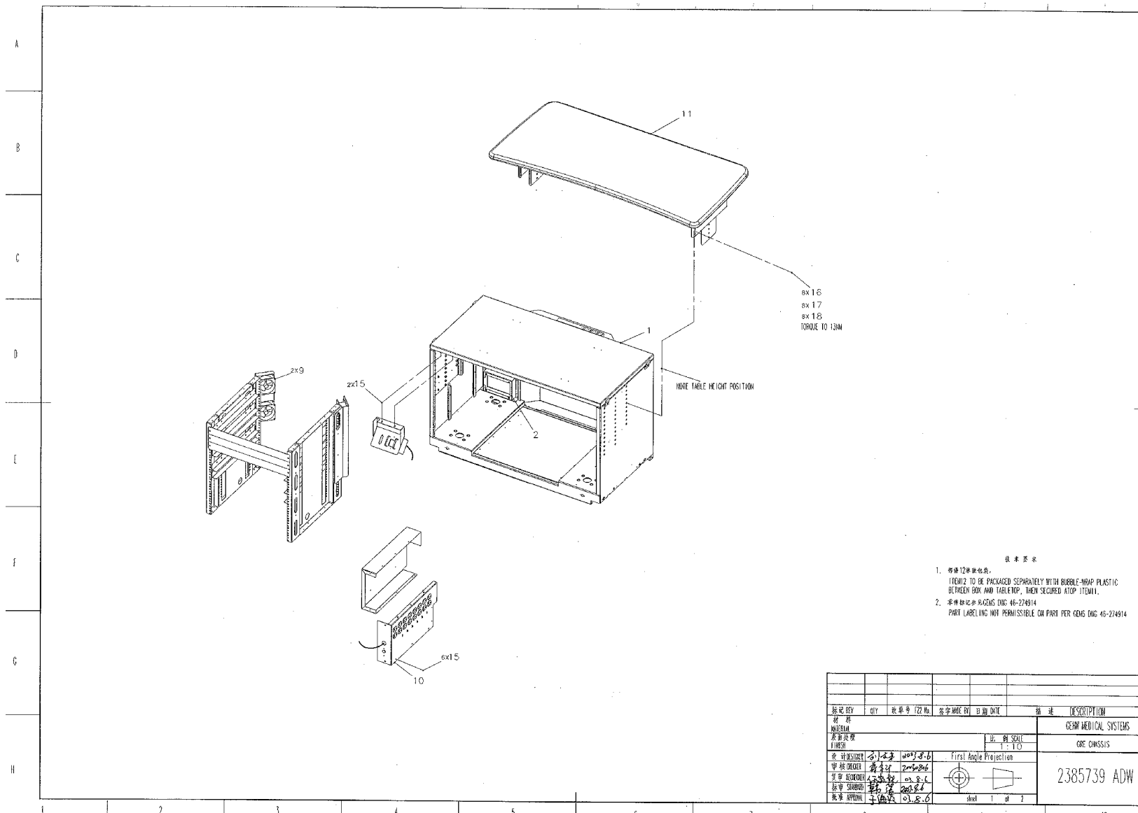
Figure 5-4 Console Chassis Assembly (2385739 sheet 1, rev 0)
