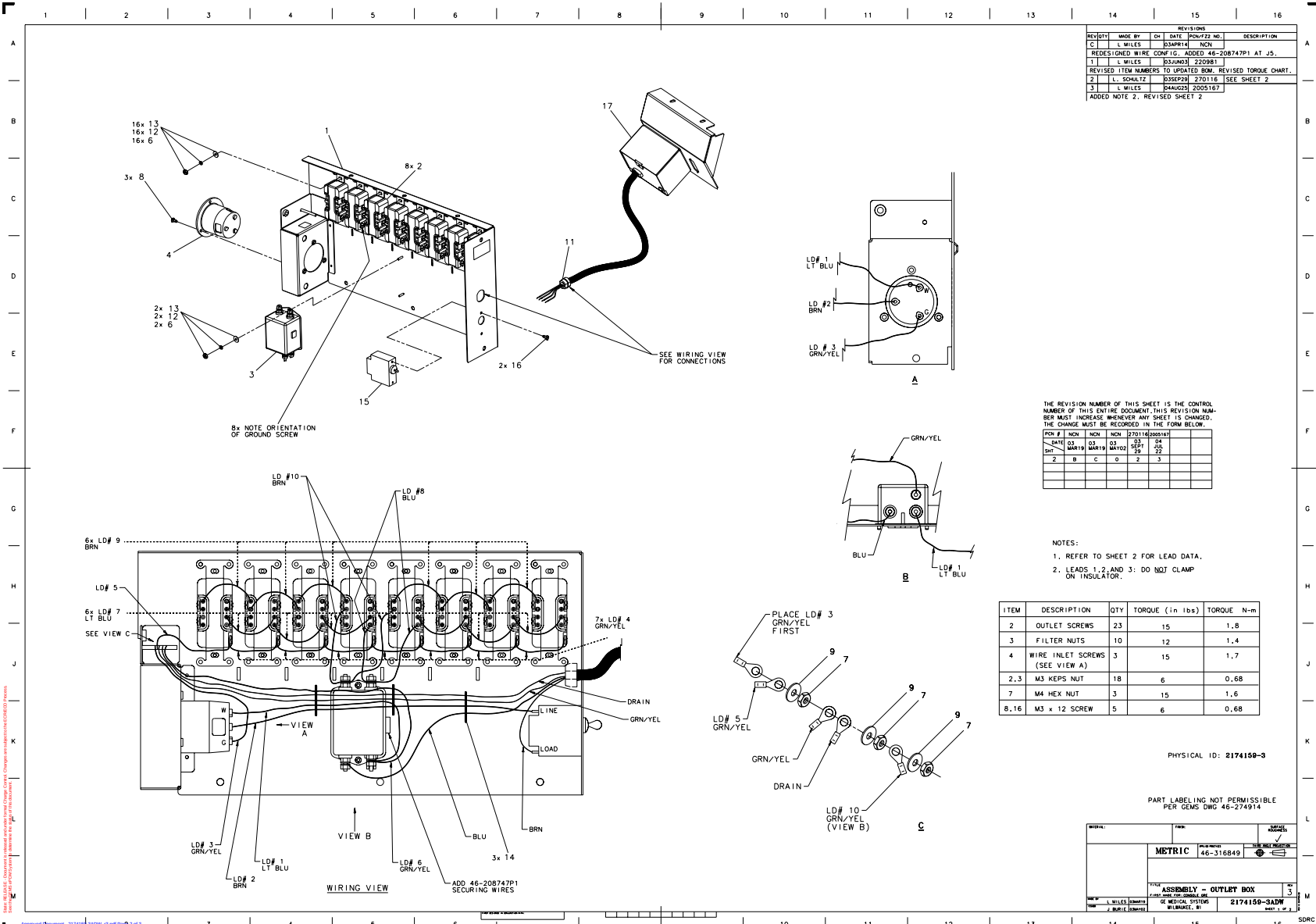
Figure 5-6 Assembly - Outlet Box (2174159-3, sheet 1, rev 3)
