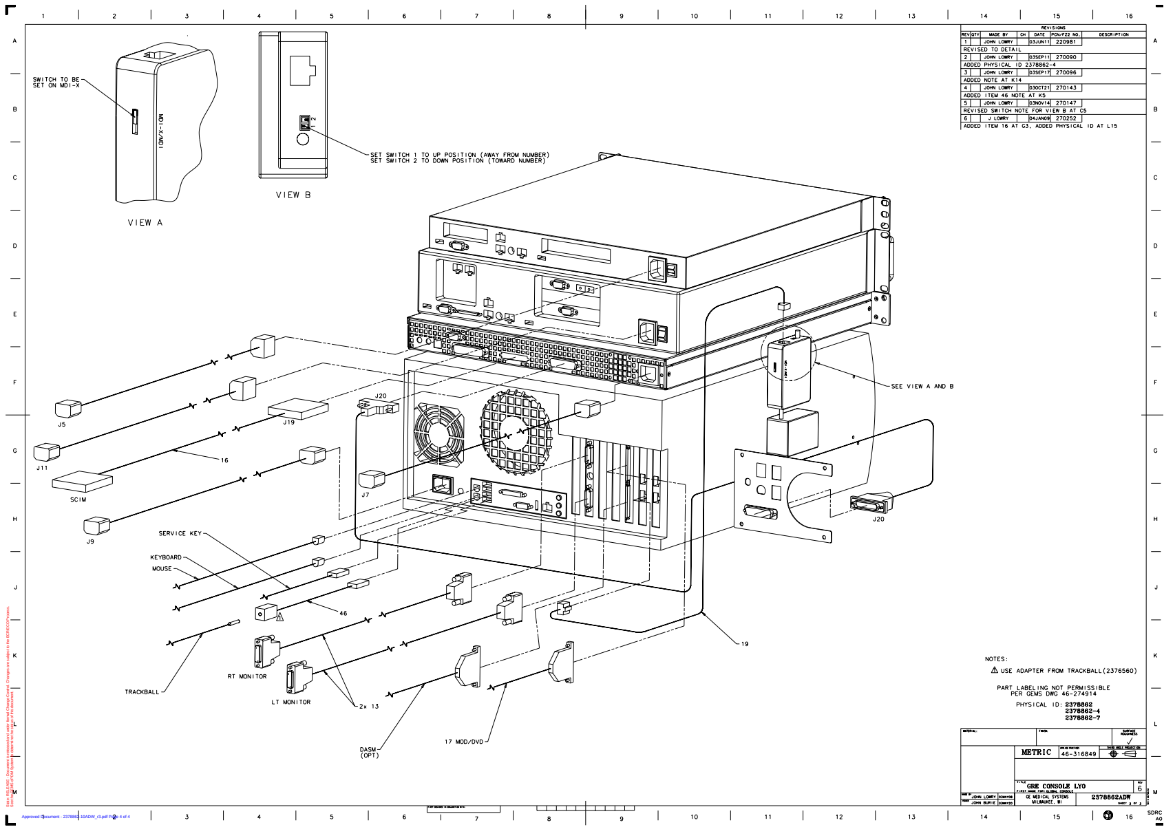
Figure 5-3 GRE Console (2378862, sheet 3, rev 06)
