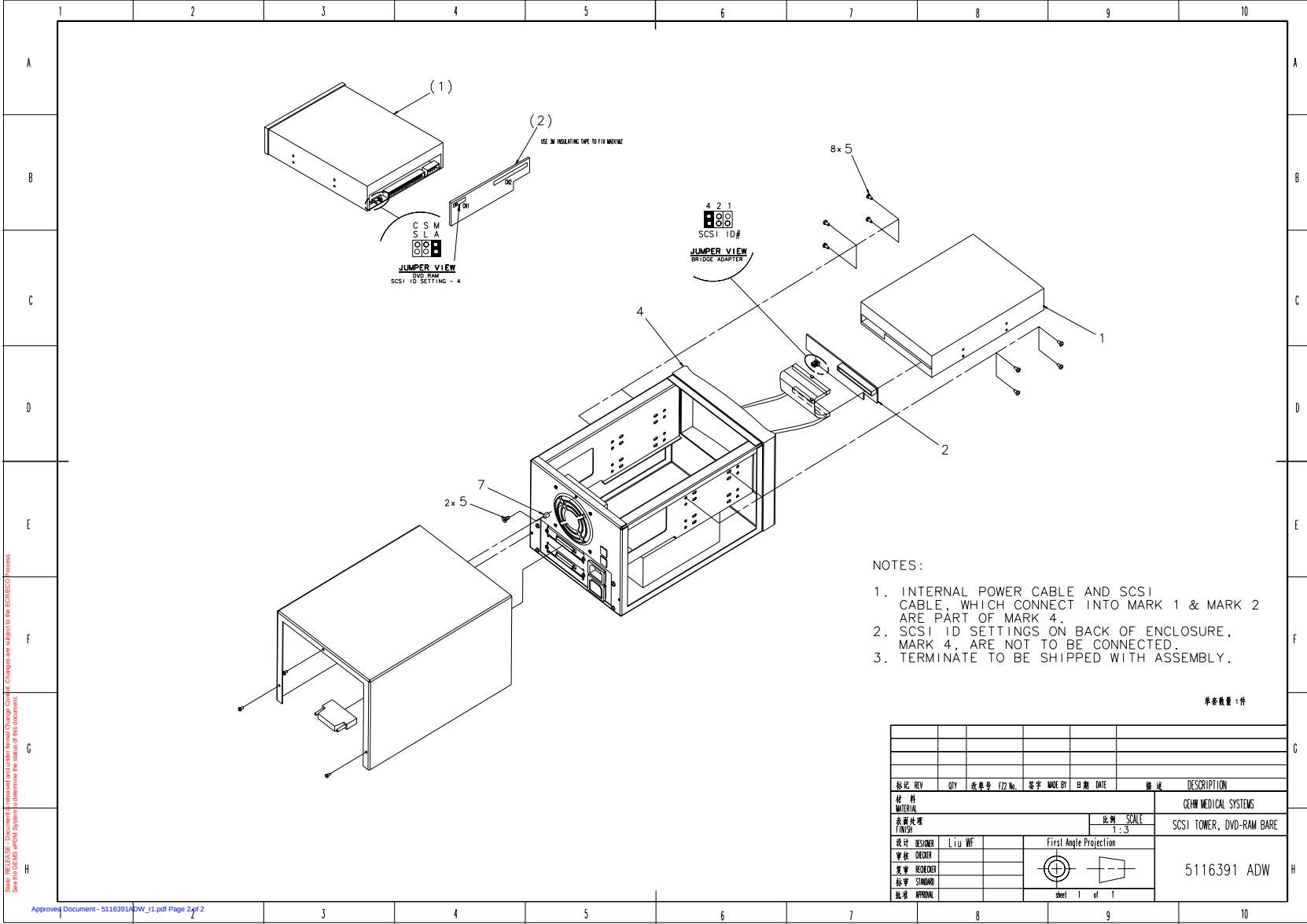
Figure 5-7 SCSI Tower, DVD-RAM, MOD (5116391, sheet 1, rev 1)
